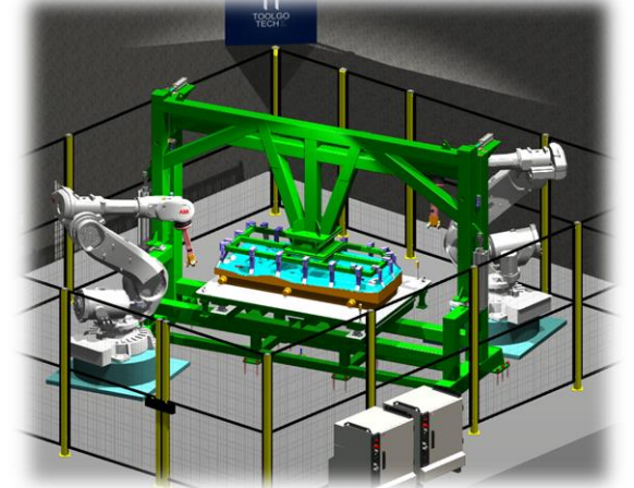
Roller Hemming Stations
