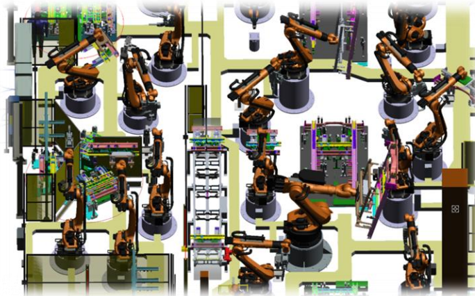
Underbody Stations
