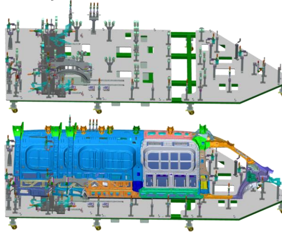
Bodyside Manual Fixture
