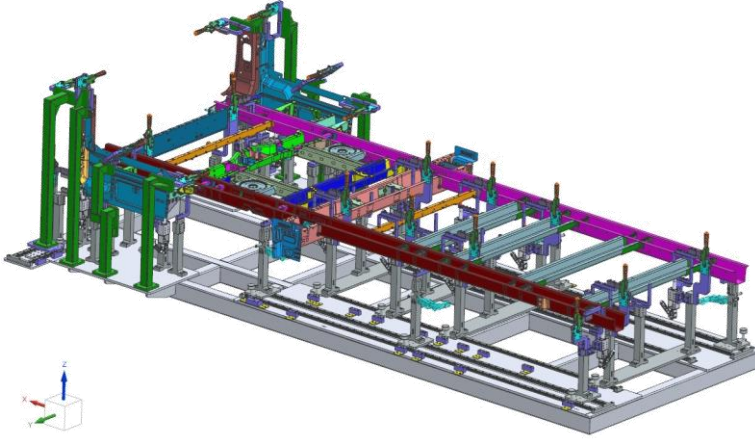
Underbody Spot Weld Fixture
